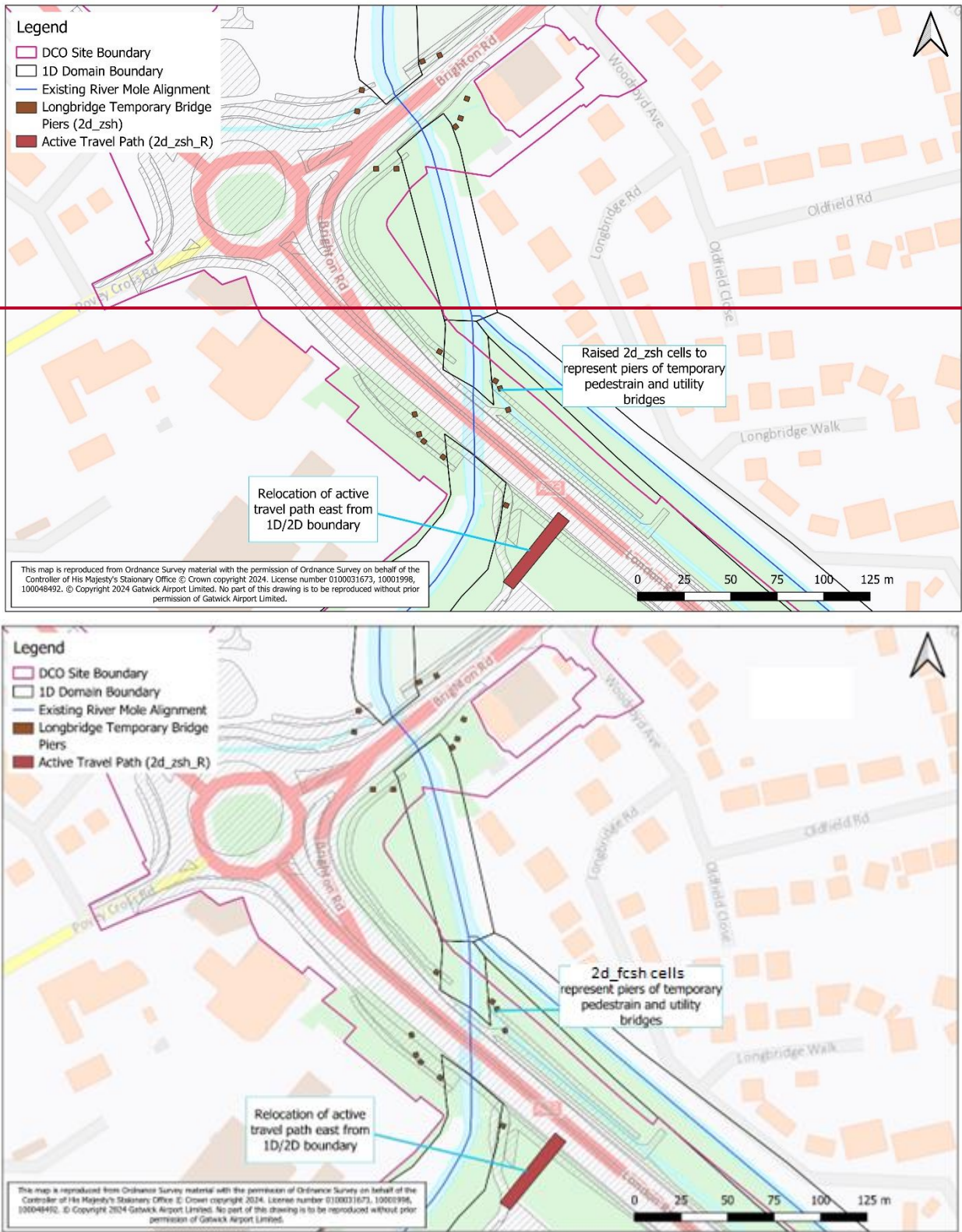
Figure 7-3: First Full Year of Opening (2029-2032) temporary bridge pier locations.
